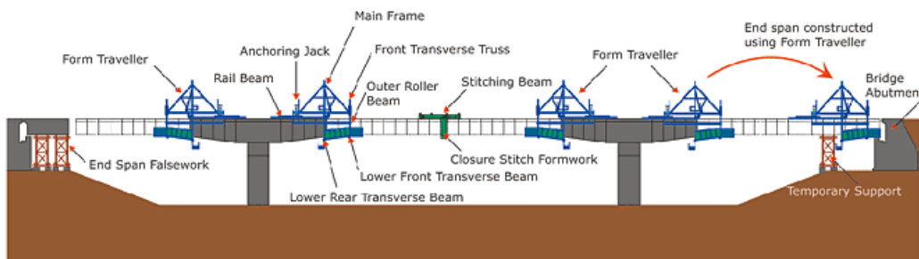
Figure 2.10: Travelling Formwork
